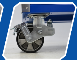
SUSPENSION CASTORS
